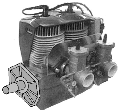
2706 - 65Hp engine shown with fan cooling
